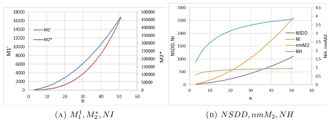
FIGURE 3. Gear graph
