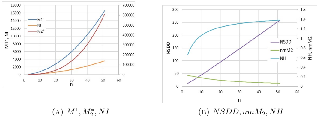
FIGURE 1. Wheel graph
