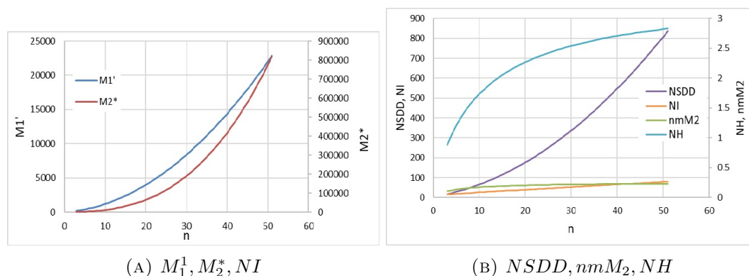
FIGURE 2. Helm graph
